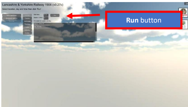
Figure 1: Startup screen
